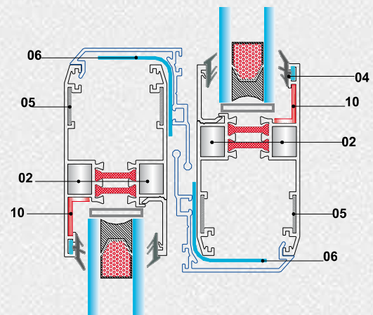
Section B
