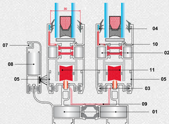
Section A
